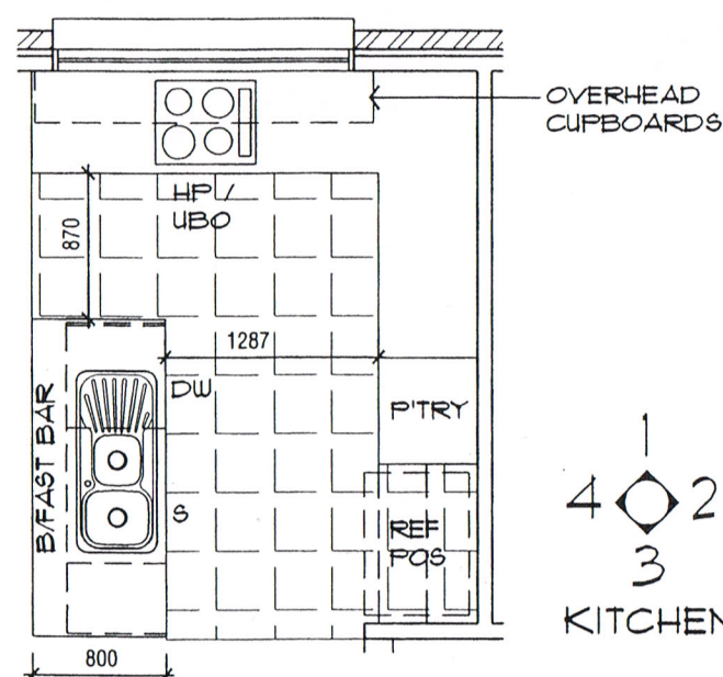
KITCHEN FLOOR PLAN
