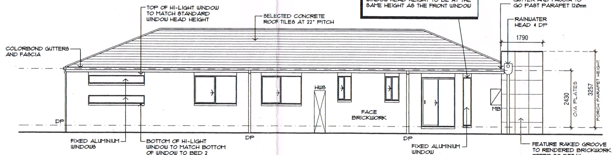
ELEVATION D
