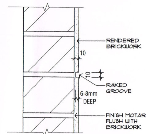
FEATURE RAKED GROOVE DETAIL SCALE 1:5
