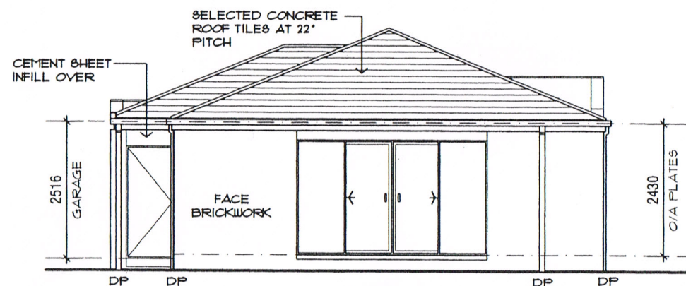
ELEVATION C
